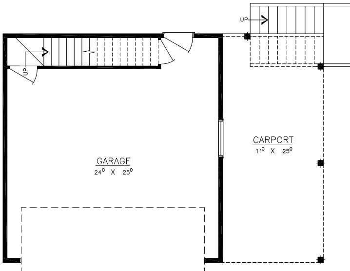
MAIN FLOOR
